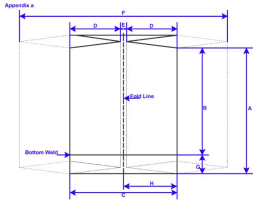
Diagram Double Gusseted / Star Sealed Bag
